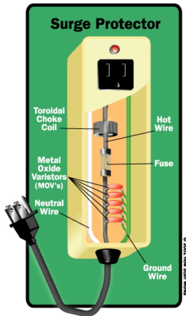
A simple MOV surge protector with line conditioning and a fuse
